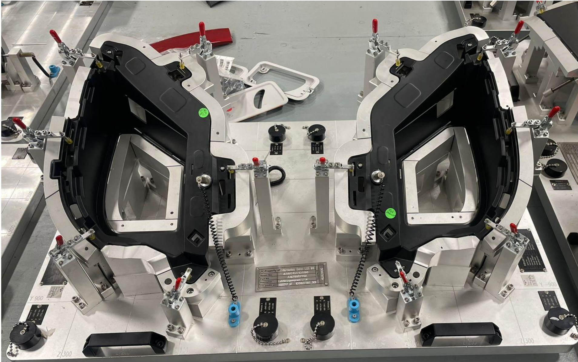
A-167-885-5706/5806 AIRDUCT SEGMENT- CHECK FIXTURE
